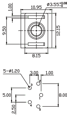
Recommended PCB Layout (PCB TOLERANCE ±0.05)
