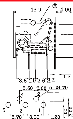
Recommended PCB Layout (PCB TOLERANCE ±0.05)
