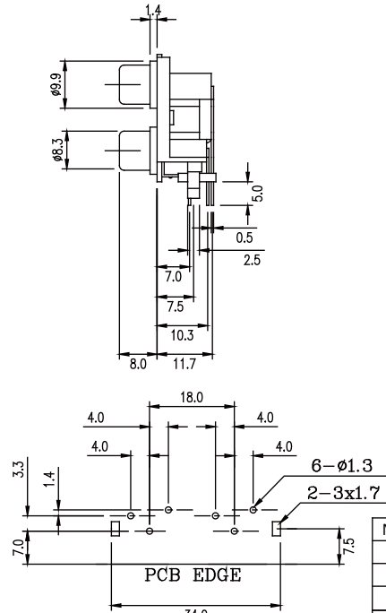
Recommended PCB Layout (PCB TOLERANCE \pm 0.05 )
