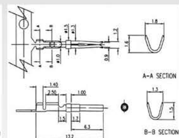
FEMALE TERMINAL:
