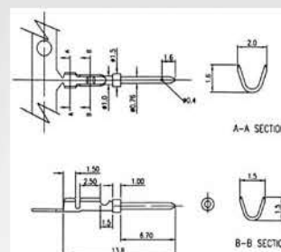
MALE TERMINAL:
