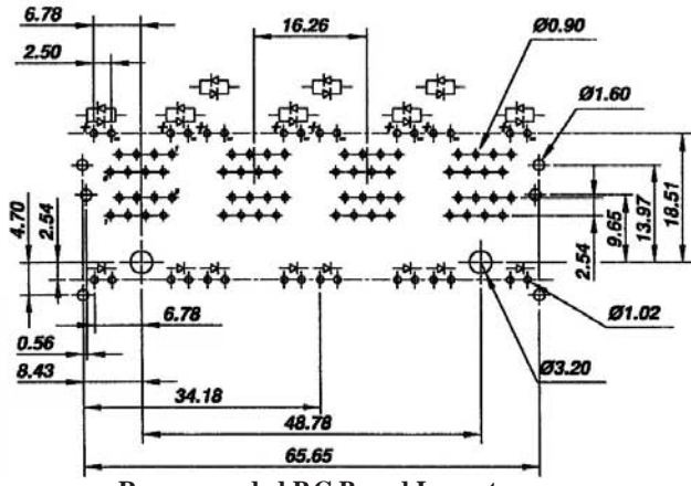
Recommended P.C. Board Layout (TOP VIEW)
