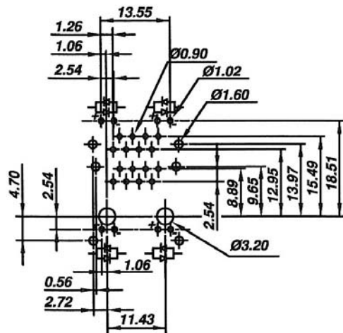
Recommended P.C.Board Layout (TOP VIEW)
