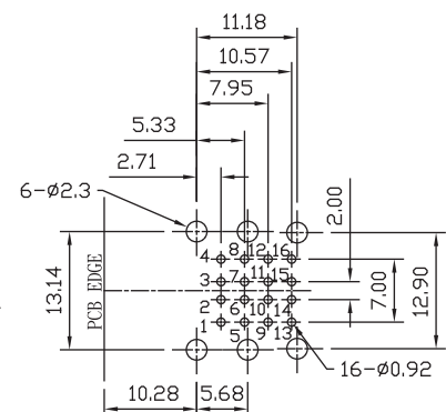
BOTTOM VIEW RECOMMENDED PCB LAYOUT
