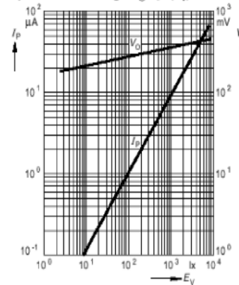
Photocurrent I_P = f(E_V) , V_R = 5 \text{ V} Open-circuit voltage V_O = f(E_V)
