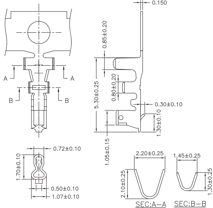
Part No.:1501-T-L
